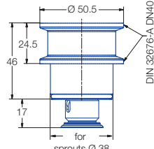
Tri-Clamp
